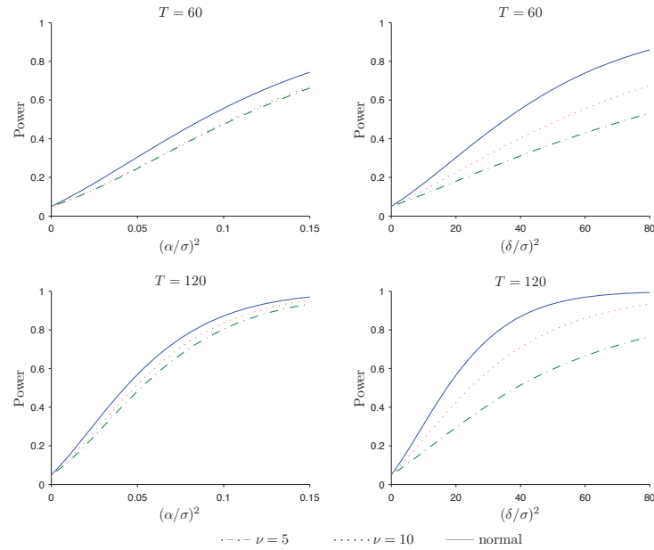
FIG. 5. Power Function of GMM Wald Test Under Multivariate Student- t Returns
