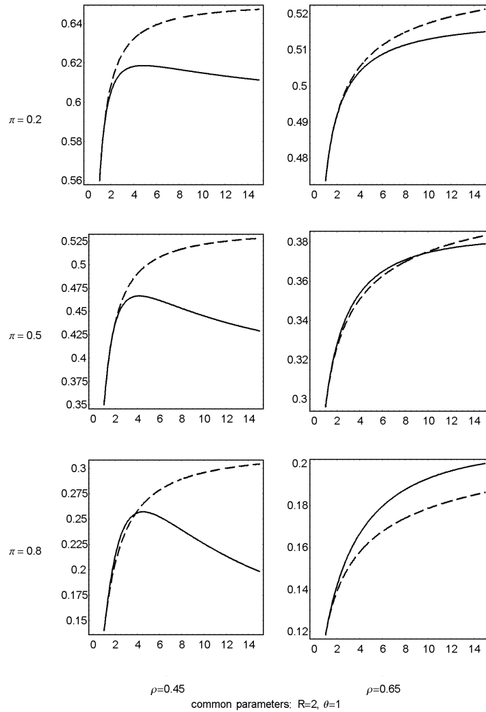
FIG. 3. Growth rates as a function of the nominal interest rate under monopoly (solid line) and competition (dashed line)
