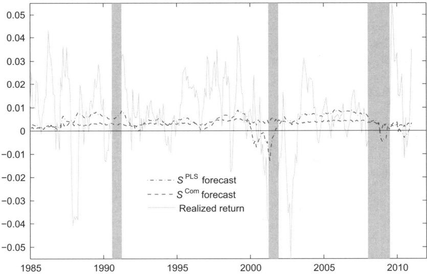
Figure 2 Excess market return forecasts of S^{PLS} and S^{Com} , January 1985 to December 2010 The dotted line depicts the out-of-sample predictive regression forecast for excess market return based on the recursively constructed aligned investor sentiment index S^{PLS} . The dashed line depicts the out-of-sample excess market return forecast based on combination forecast S^{Com} as the simple equally-weighted average of univariate predictive regression forecasts. The solid line depicts the excess market return smoothed with six month moving average. The sentiment indices and excess market return forecasts are estimated recursively based on information up to the period of forecast formation period t alone. The vertical bars correspond to NBER-dated recessions.
